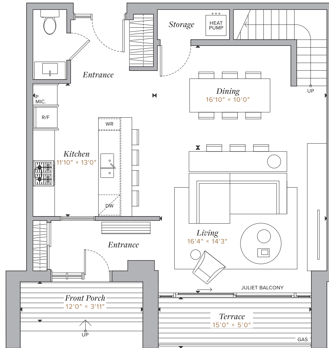
Ground Floor
